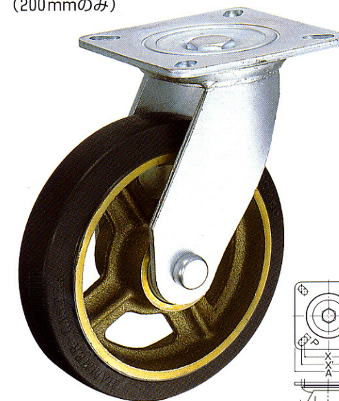
500HPS-CR 200mm
