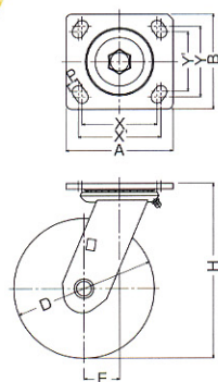
500BPS-CU 150mm
